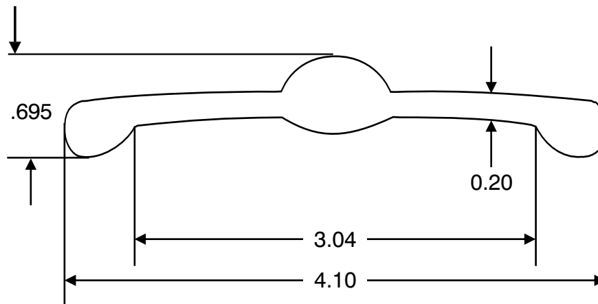
The Hybrid 3-Rail's Flex Curve™
